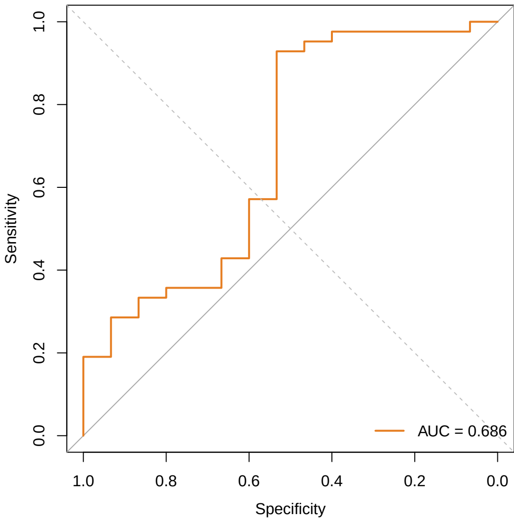
ROC Curve (AUC = 0.686 )
